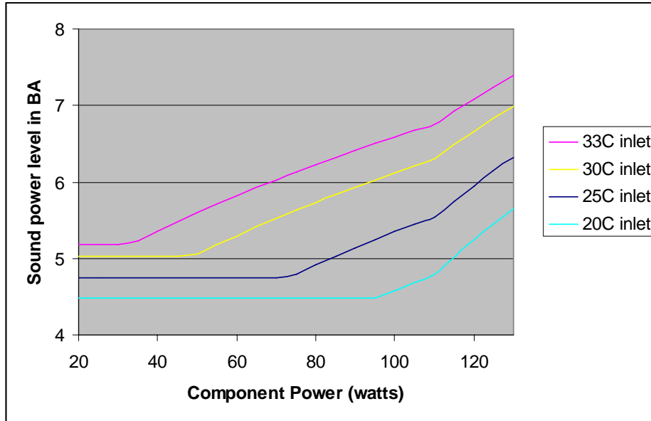
Figure 2 Sound power vs. component power at four system ambient temperature conditions
