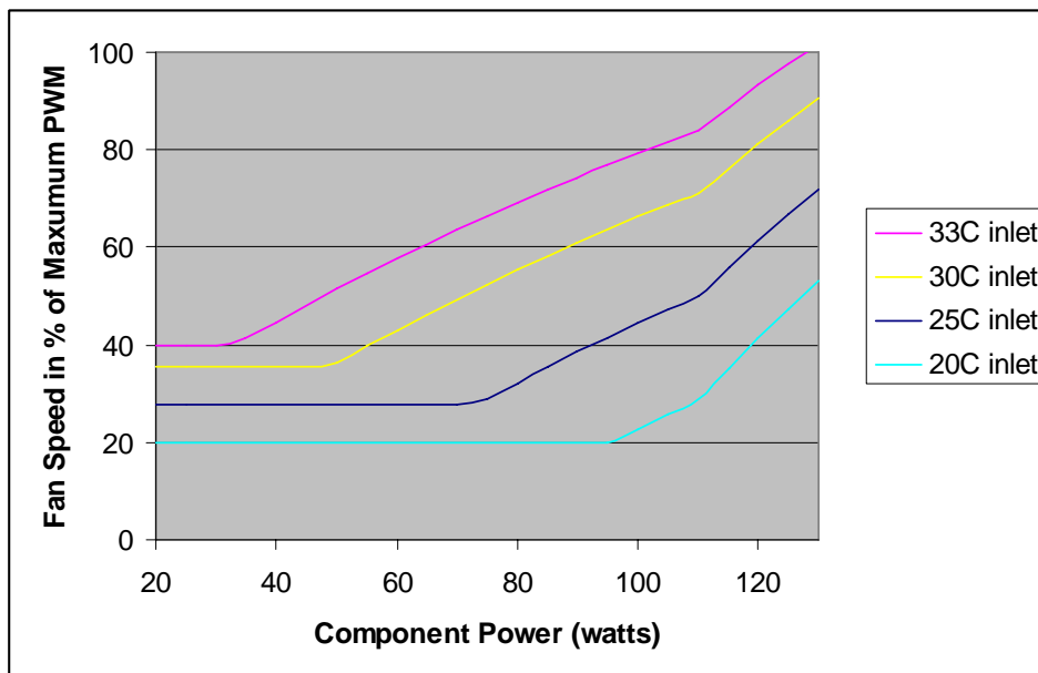
Figure 1 Fan speed vs. component power at four system ambient temperature conditions
