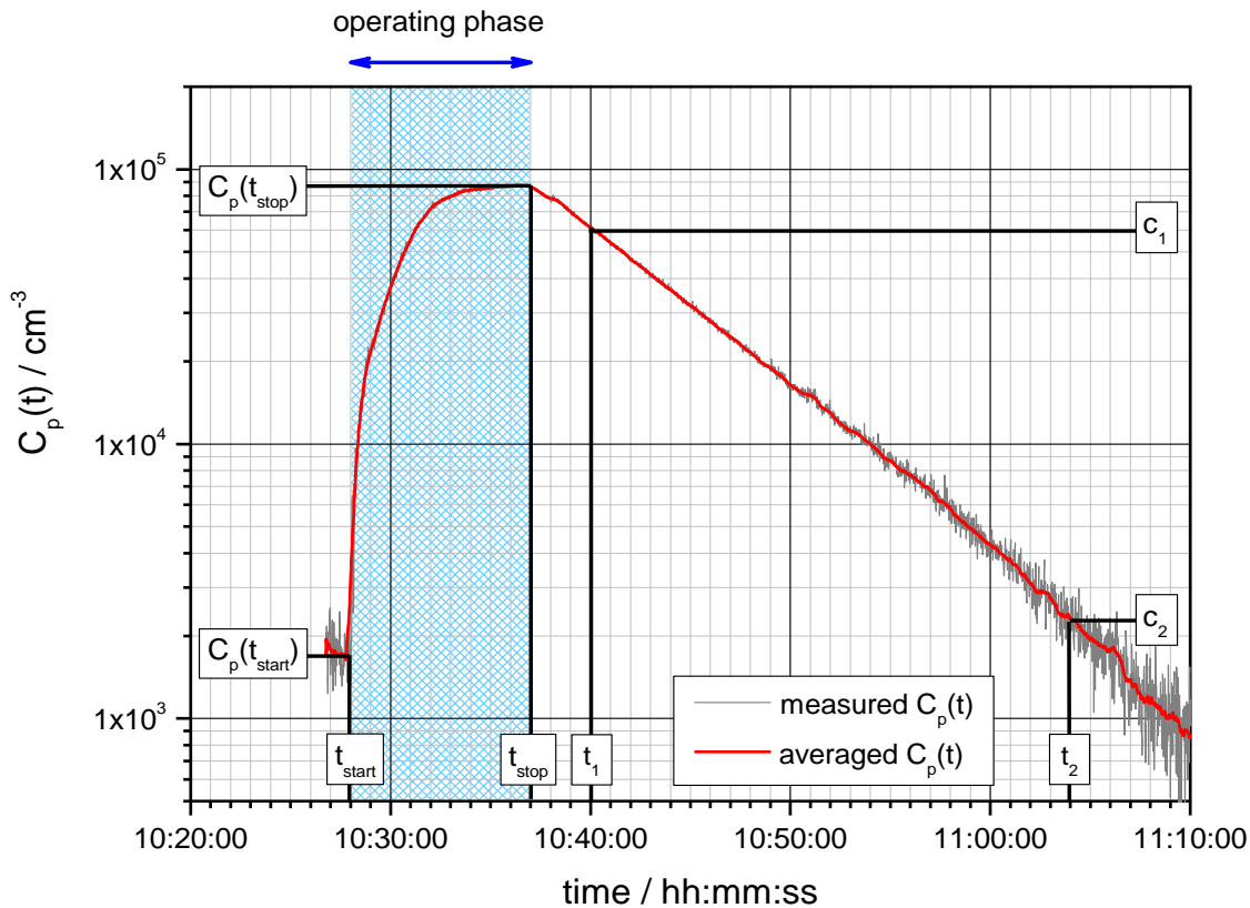
Figure 6 — Diagram of a total particle number concentration time series (example)
