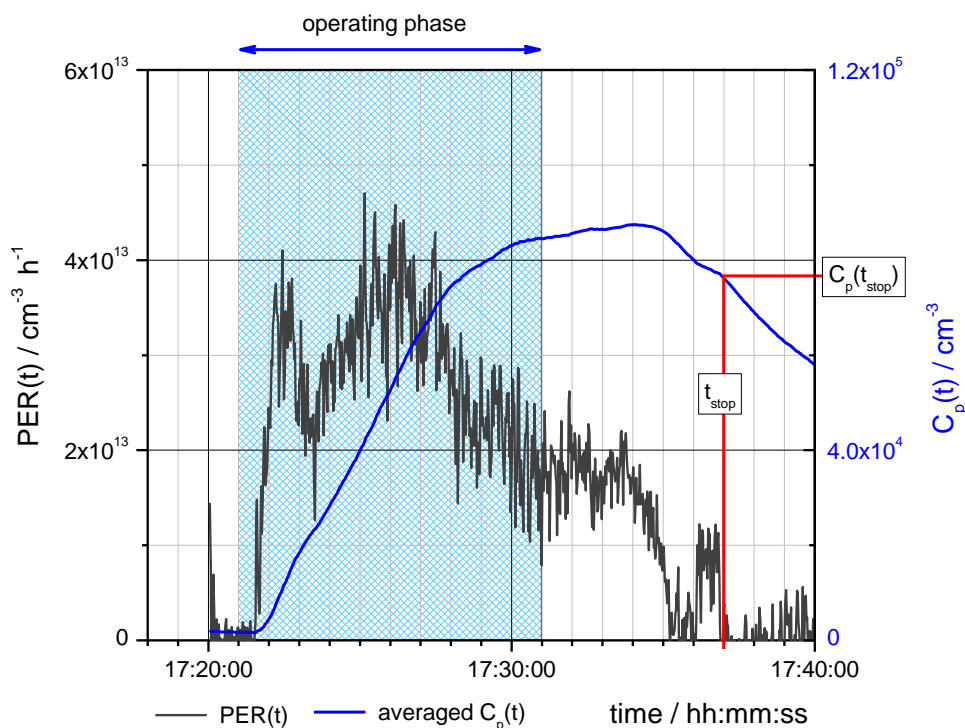
Figure 7 — Diagram of PER(t) and C_p(t)
