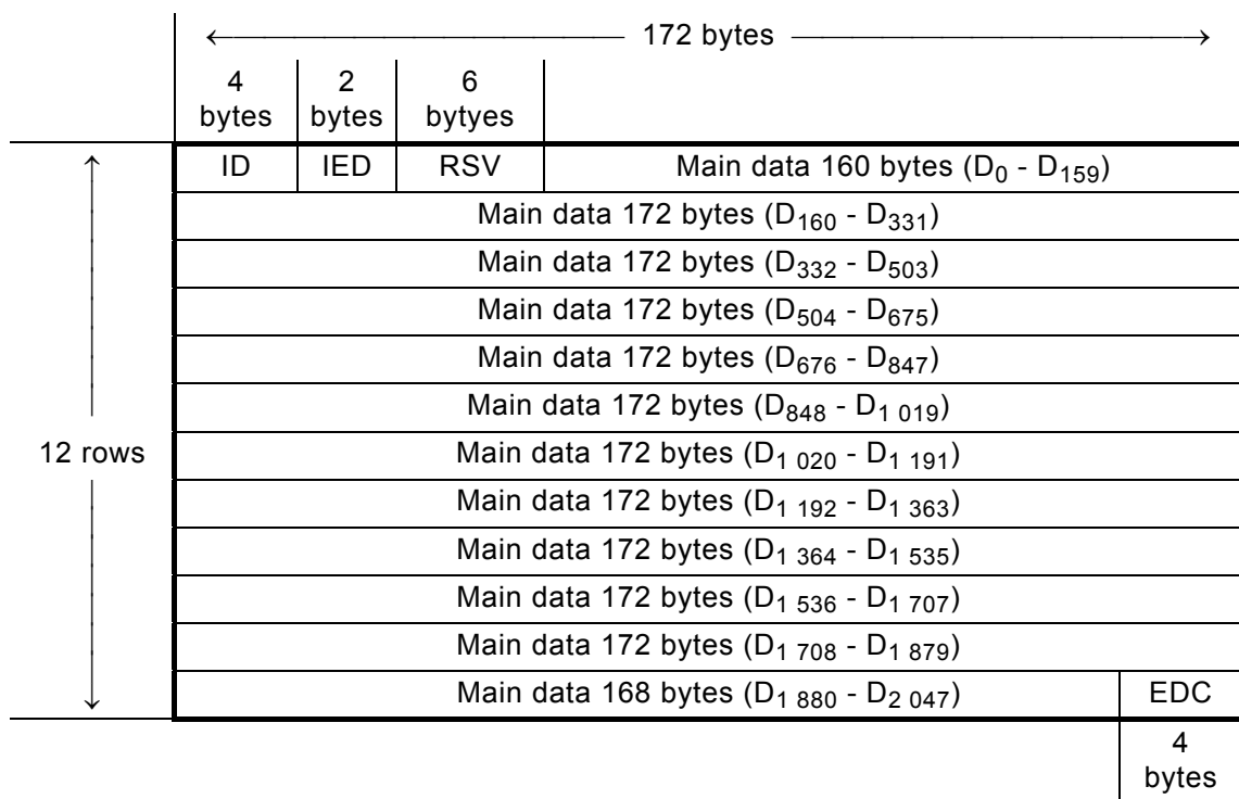
Figure 10 — Data Frame
