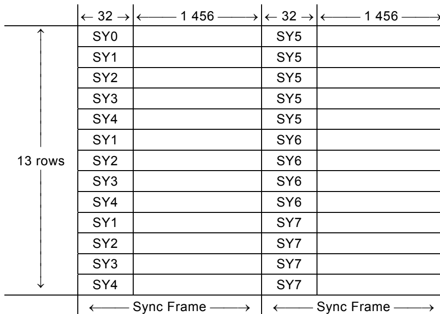
Figure 16 — Physical Sector
