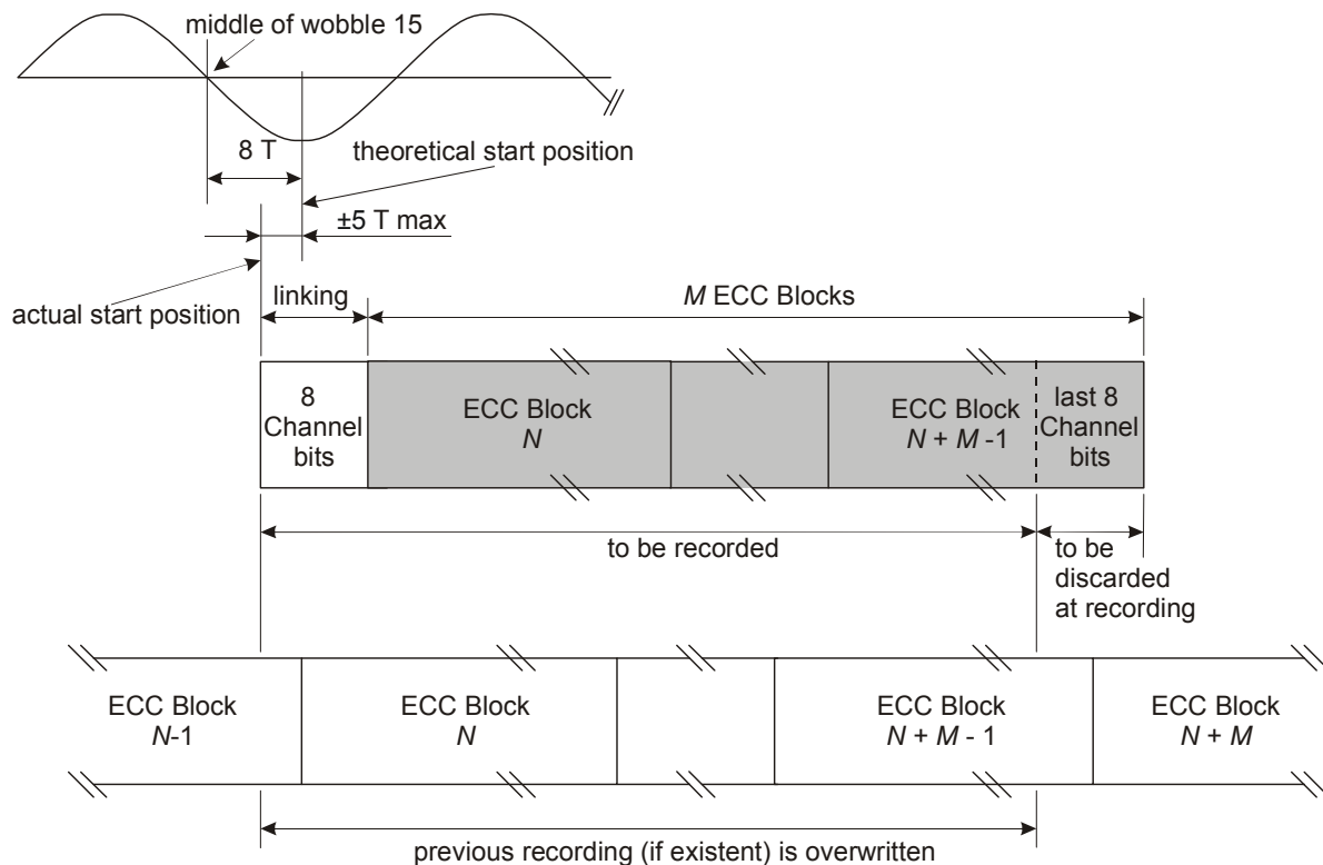
Figure 17 — Recording Unit
