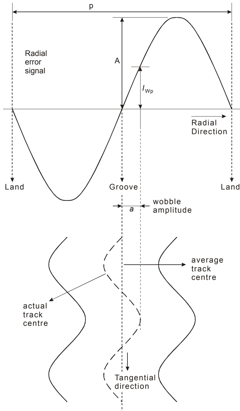
Figure K.1 — Wobble amplitude of the groove
