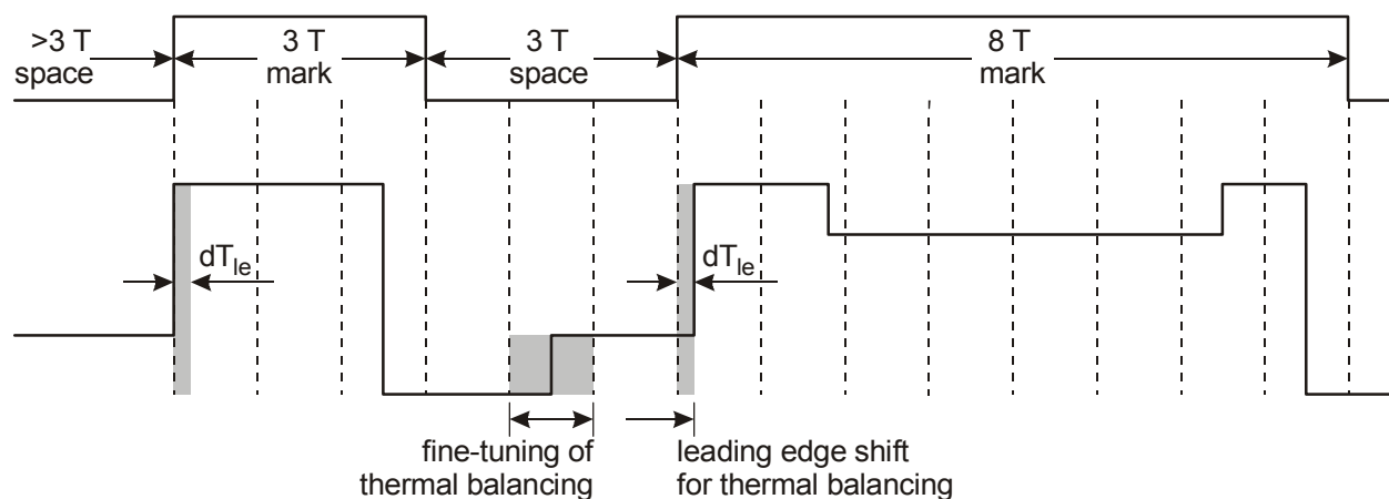
Figure G.6 — Example of a Castle waveform
