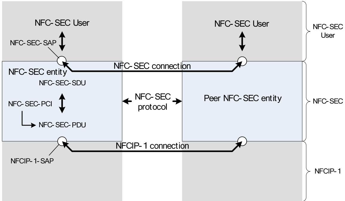
Figure 1 – NFC-SEC architecture
