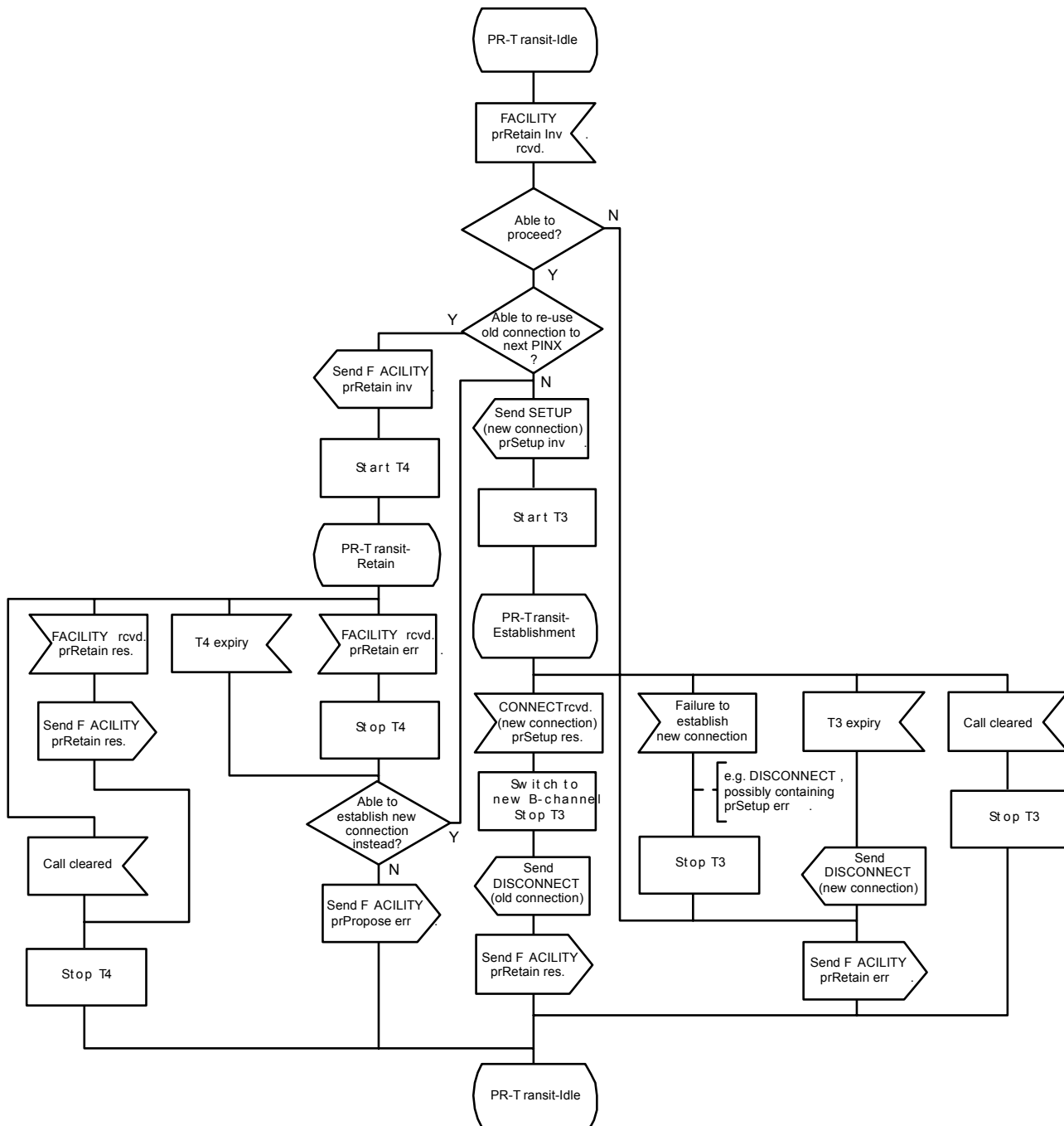
Figure D.4 - Transit PINX SDL
