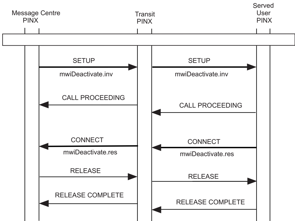
Figure B.2 - Example of deactivation of SS-MWI
