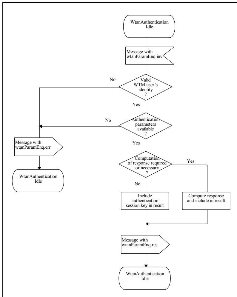
Figure D.9 - SDL representation of SS-WTAN at the Authentication Server PINX
