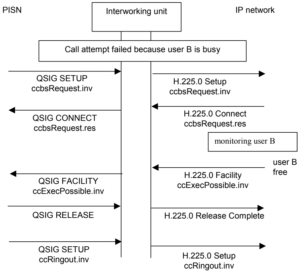
Figure B.2 – Example of scenario A1: successful call completion on busy, connection retention option
