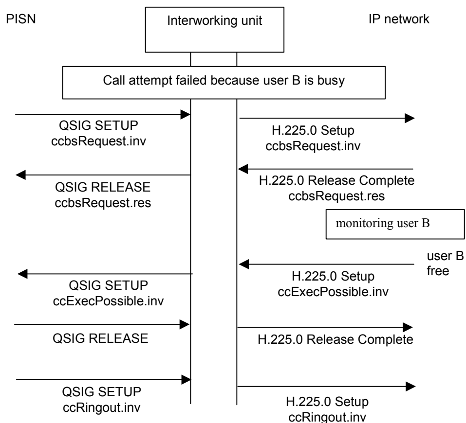
Figure B.1 – Example of scenario A1: successful call completion on busy, connection release option
