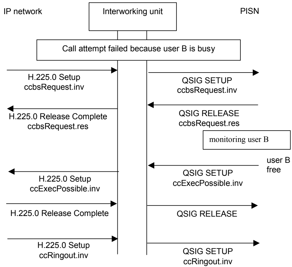
Figure B.3 – Example of scenario A2: successful call completion on busy, connection release option
