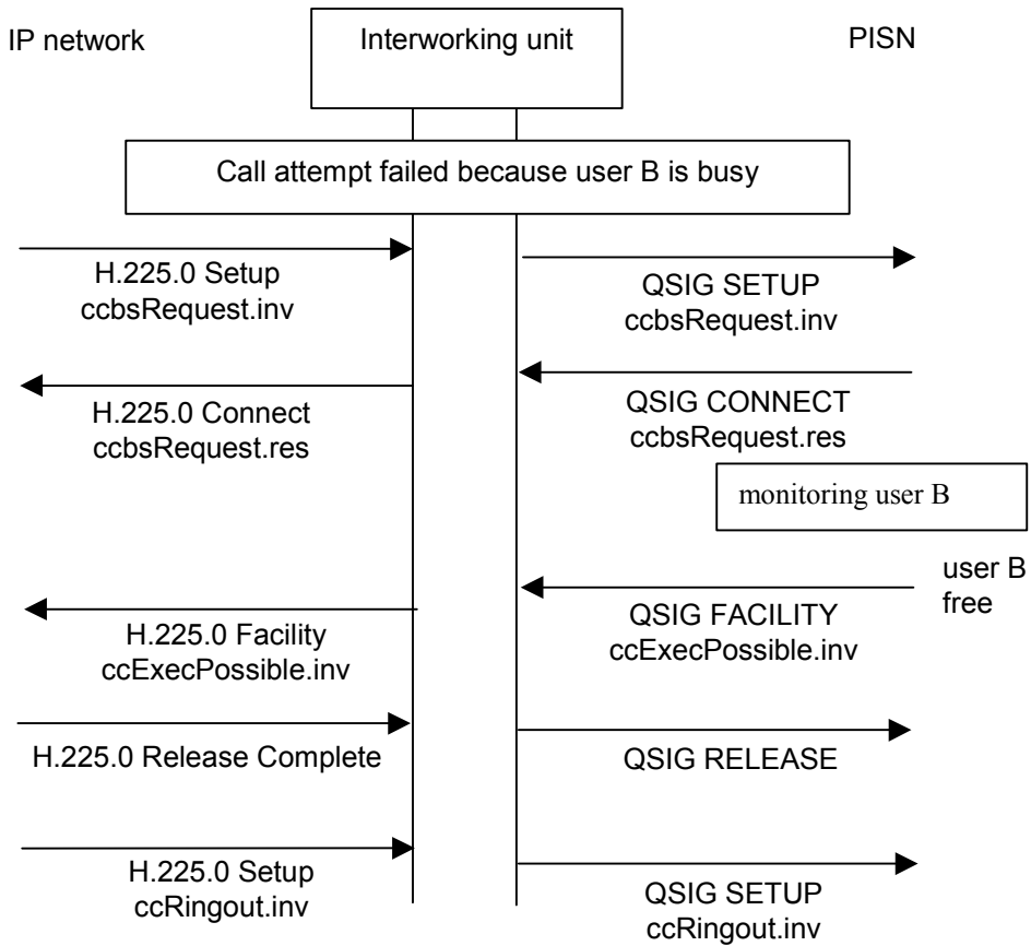
Figure B.4 – Example of scenario A2: successful call completion on busy, connection retention option
