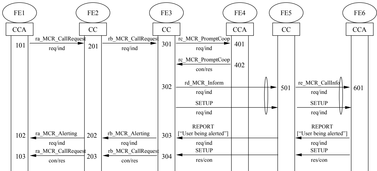
Figure 3 – Information flow sequence for invocation of SS-MCR
