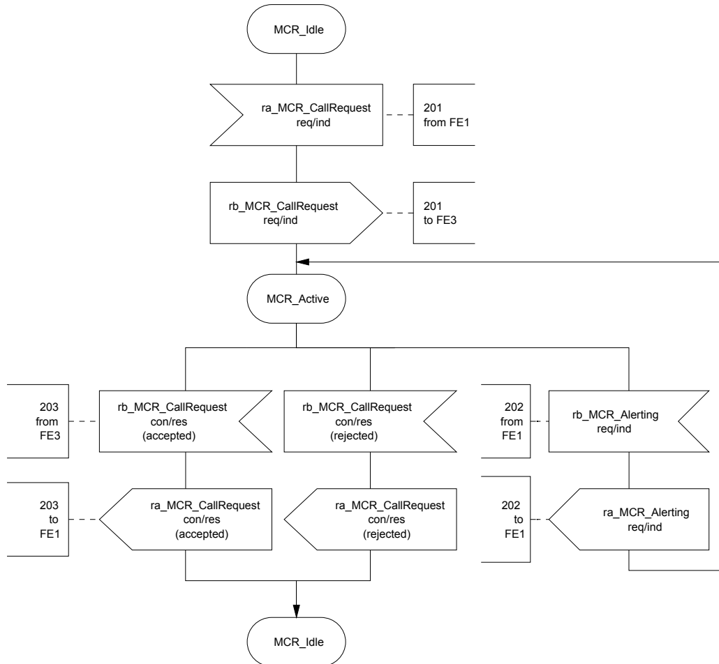
Figure 5 – SDL for MCR Procedures for FE2, Requesting User's control entity
