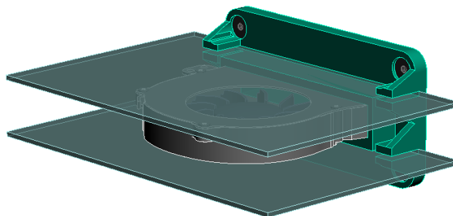
Figure 17 — Complete test fixture with inlet restriction plates
