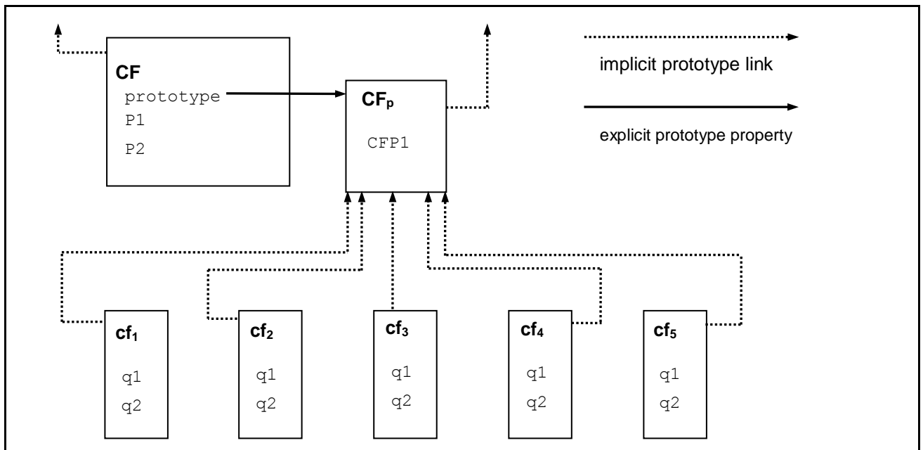
Figure 1 — Object/Prototype Relationships
