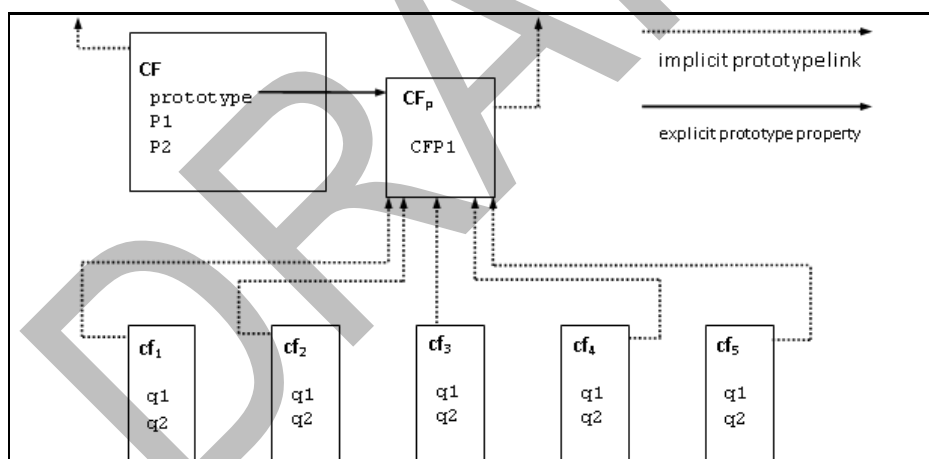
Figure 1 — Object/Prototype Relationships
