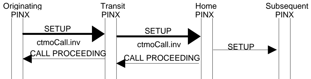
Figure B.2 - Successful invocation of ANF-CTMO with en-bloc operation
