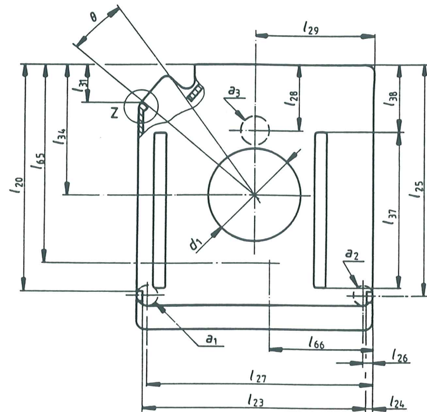
Figure 5 - Bottom side of case
