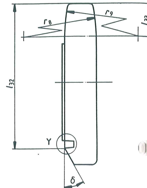
Figure 6 - Side of case
