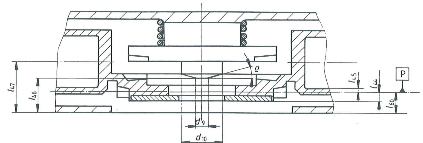
Figure 11 - Cross-section of the cartridge in the drive
