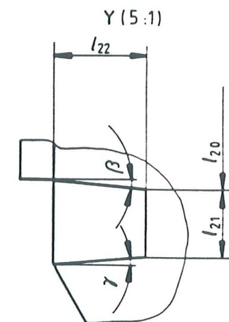
Figure 8 - Cross-section of a location notch
