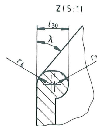
Figure 9 - Cross-section of a detail of the opening of case
