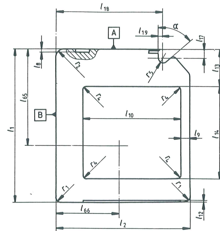
Figure 3 - Top side of case
