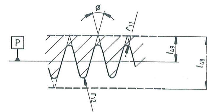
Figure 12 - Teeth of the toothed rim
