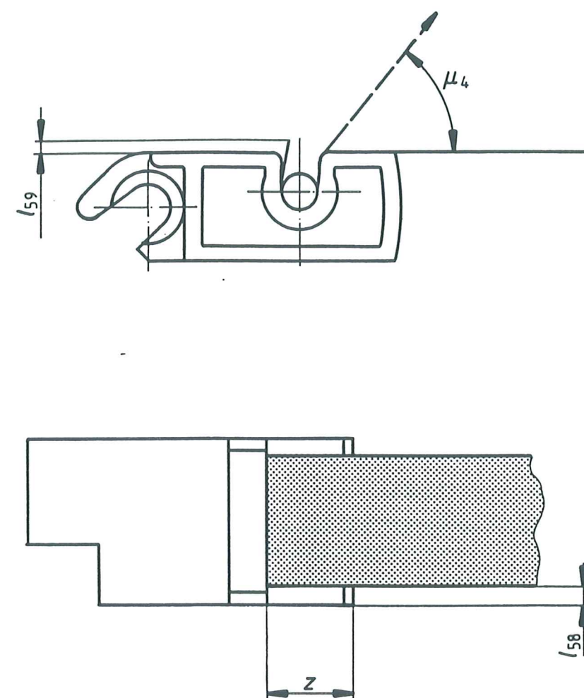
Figure 14 - Fixation of tape to leader block
