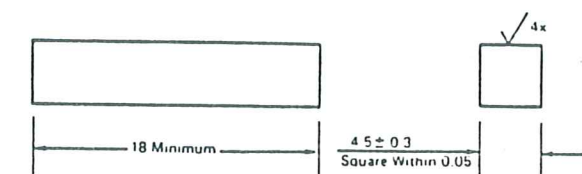
Figure C1 - Ferrite Wear Bar
