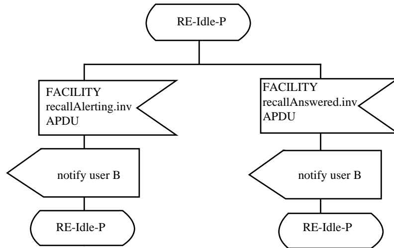
Figure C.2 - SDL for Primary PINX
