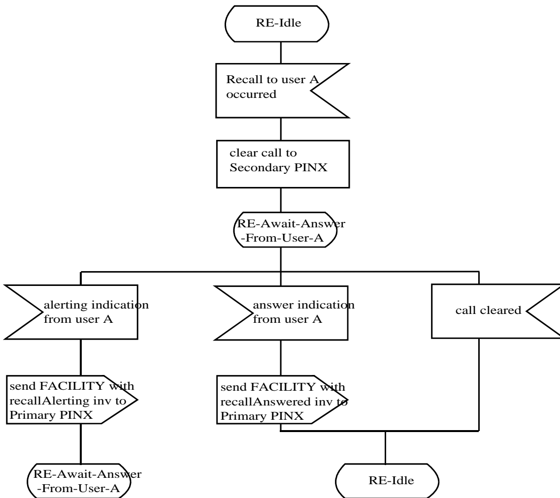
Figure C.1 - SDL for Served User PINX
