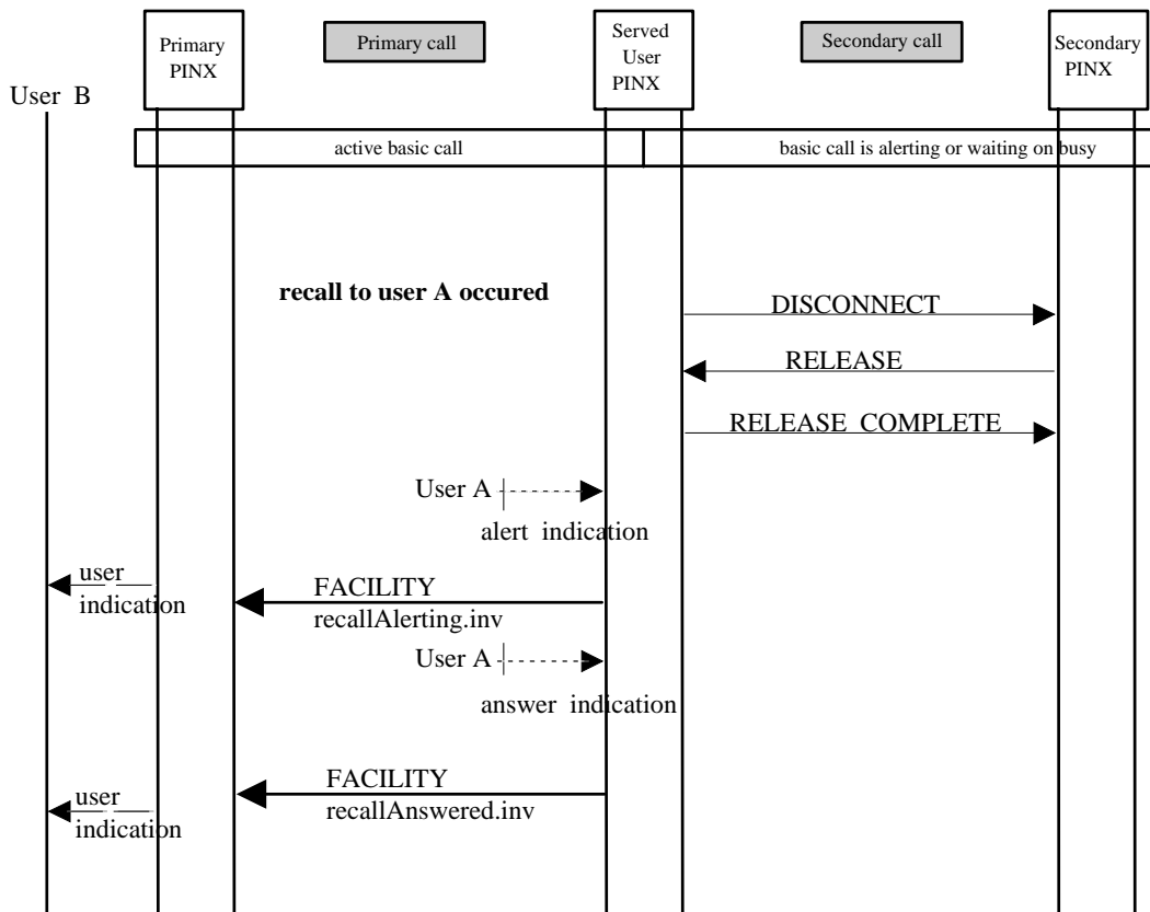
Figure B.1.1 - Successful invocation of SS-RE
