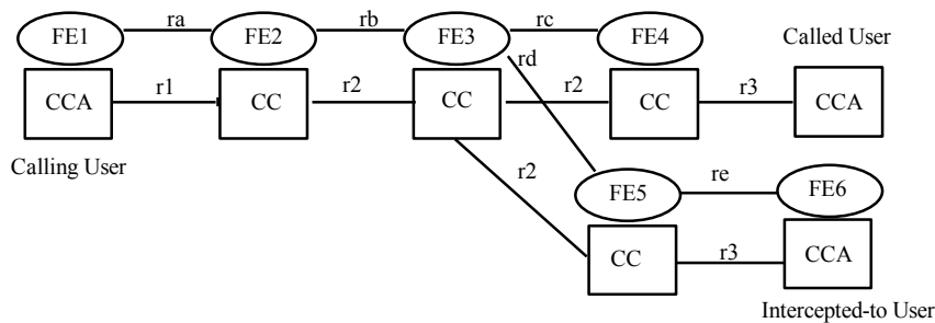
Figure 3 - Example relationship between model for ANF-CINT and basic call
