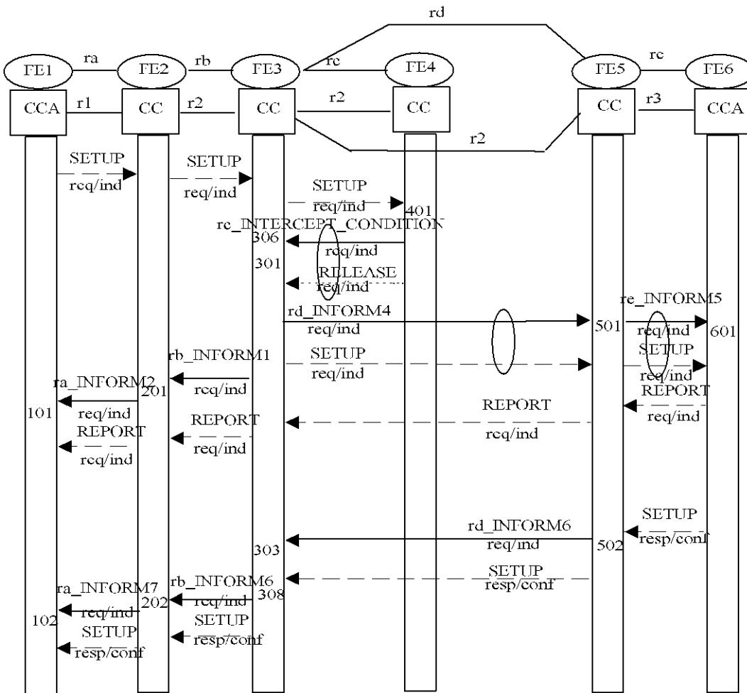
Figure 4 - Information flow sequence - successful invocation of interception immediate
