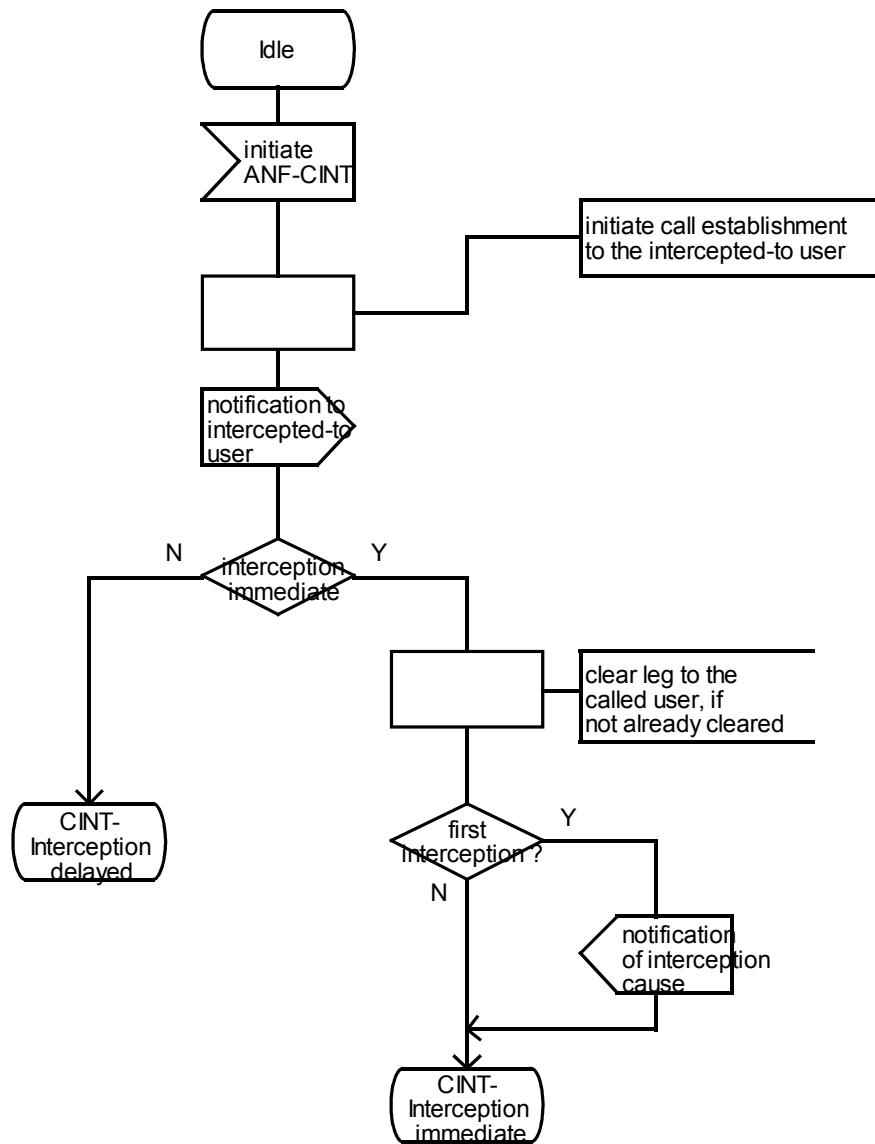
Figure 1 - ANF-CINT, overall SDL (part 1)
