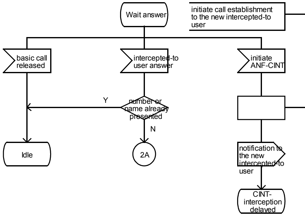
Figure 1 - ANF-CINT, overall SDL (part 4)
