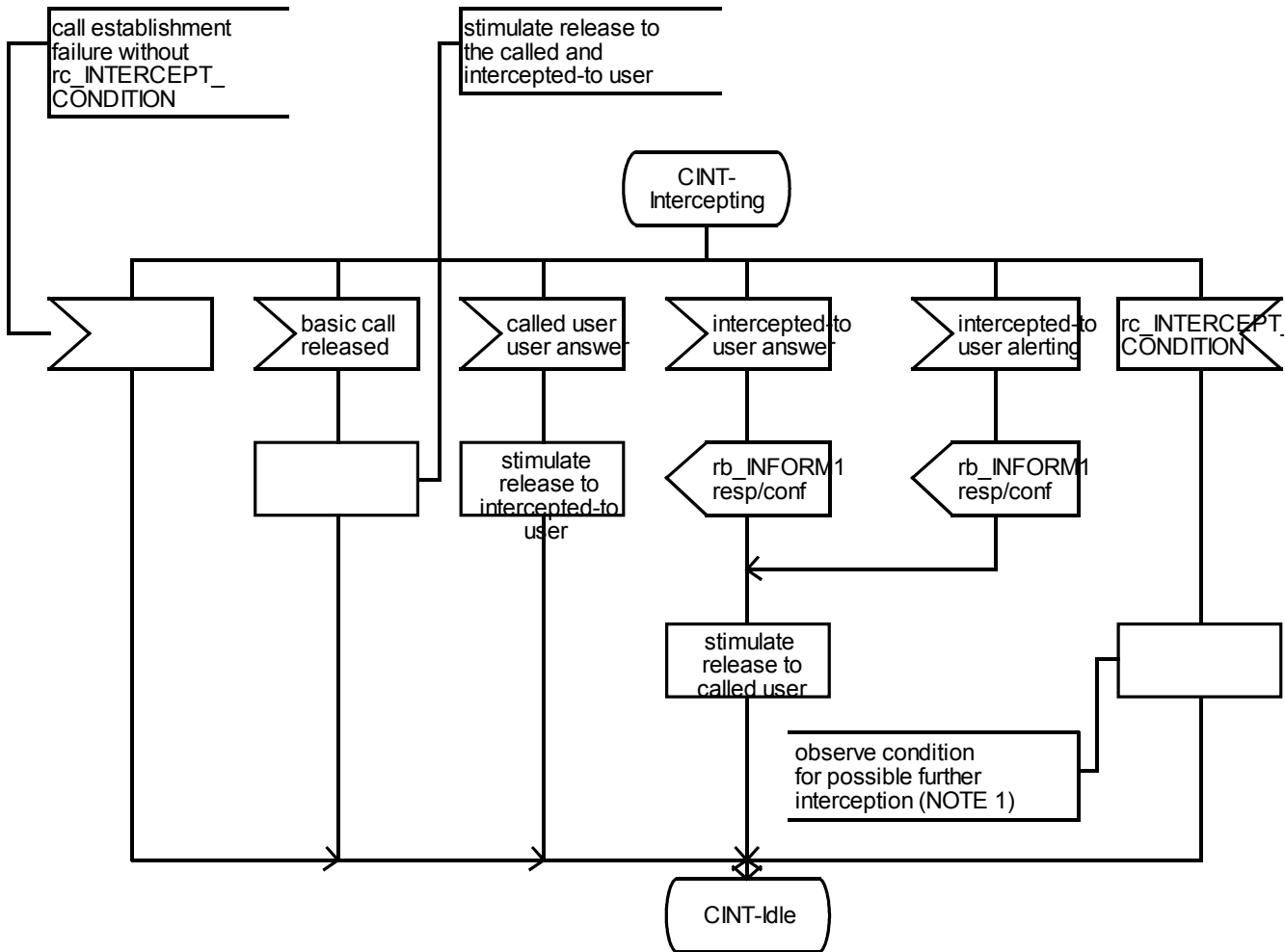
Figure 13 - ANF-CINT, SDL for functional entity FE3 (part 2)
