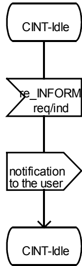
Figure 16 - ANF-CINT, SDL for functional entity FE6
