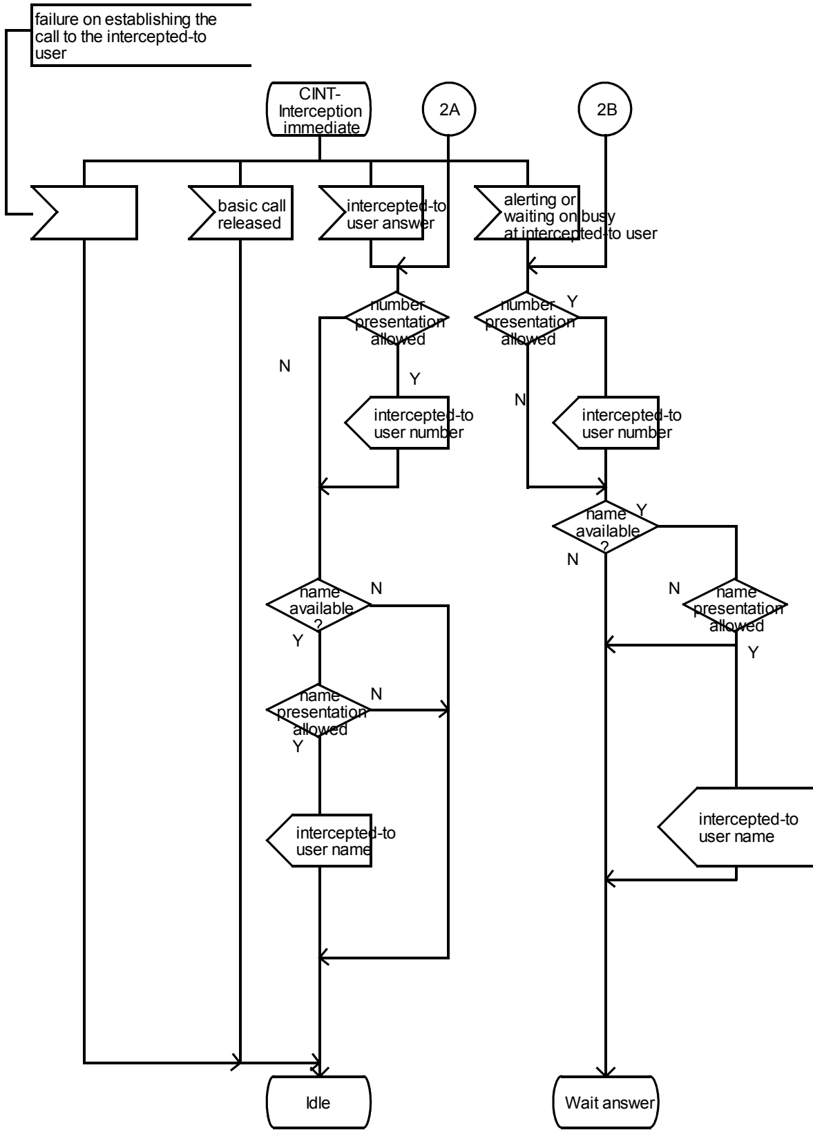
Figure 1 - ANF-CINT, overall SDL (part 2)
