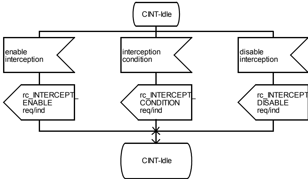
Figure 14 - ANF-CINT, SDL for functional entity FE4
