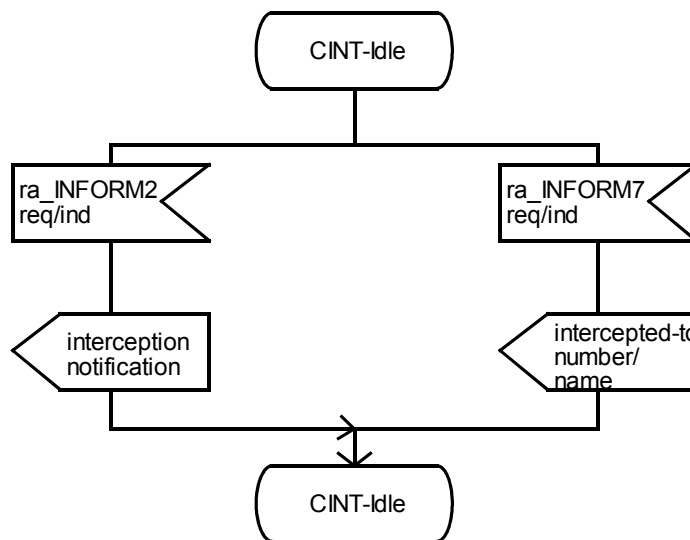
Figure 11 - ANF-CINT, SDL for functional entity FE1
