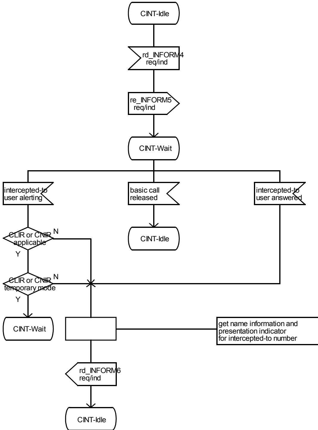
Figure 15 - ANF-CINT, SDL for functional entity FE5
