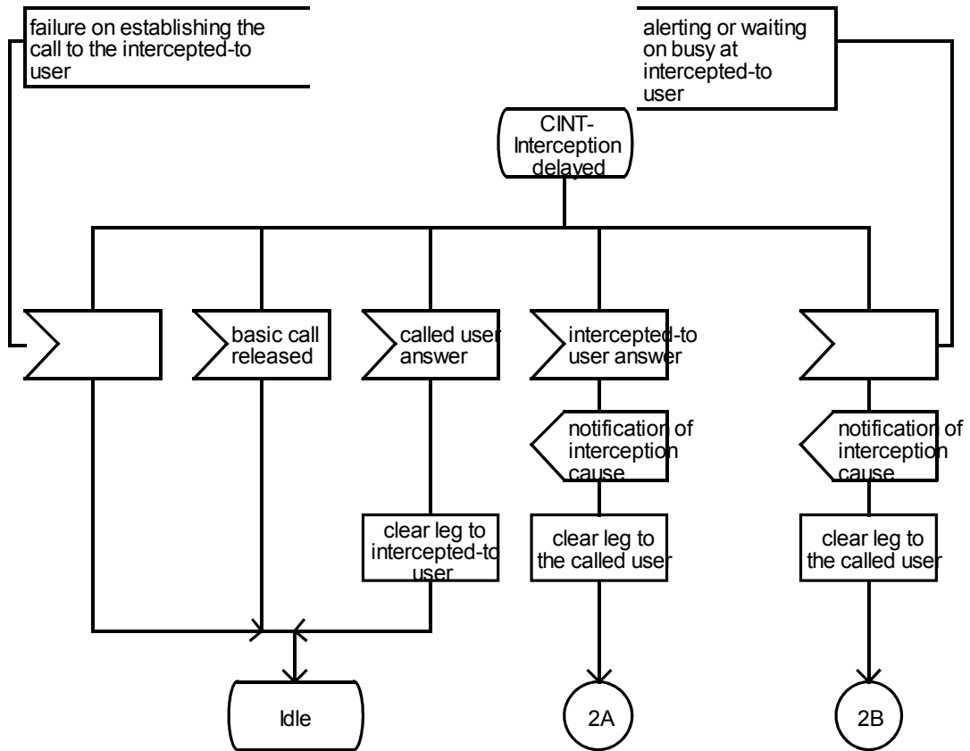
Figure 1 - ANF-CINT, overall SDL (part 3)
