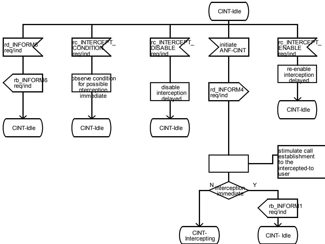
Figure 13 - ANF-CINT, SDL for functional entity FE3 (part 1)
