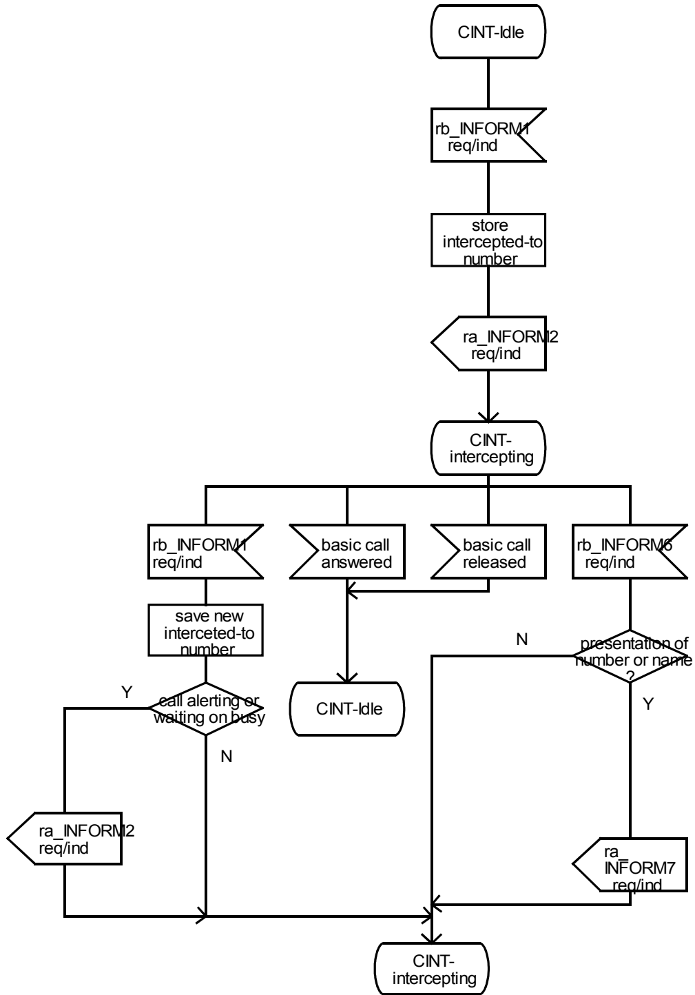
Figure 12 - ANF-CINT, SDL for functional entity FE2
