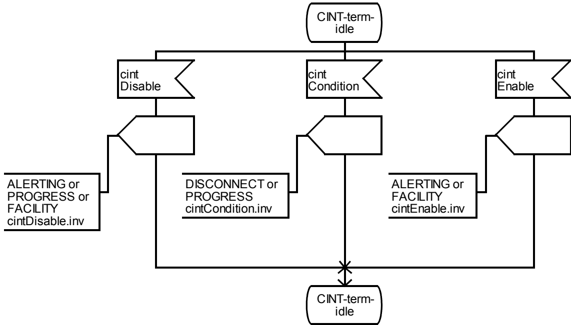
Figure C.4 - SDL Representation of ANF-CINT at the Terminating PINX
