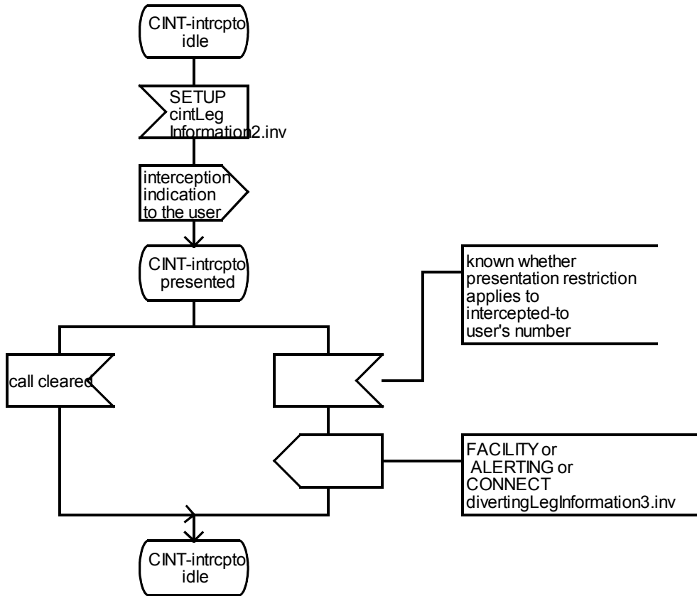
Figure C.3 - SDL Representation of ANF-CINT at the Intercepted-to PINX
