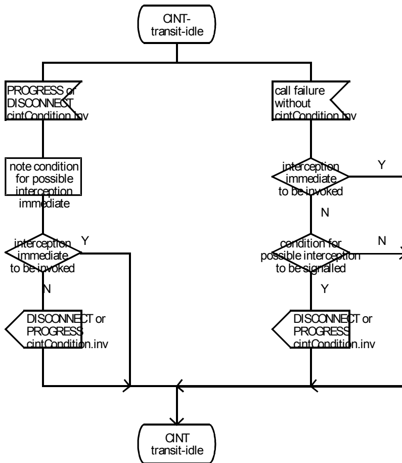
Figure C.5 - SDL Representation of ANF-CINT at a Transit PINX
