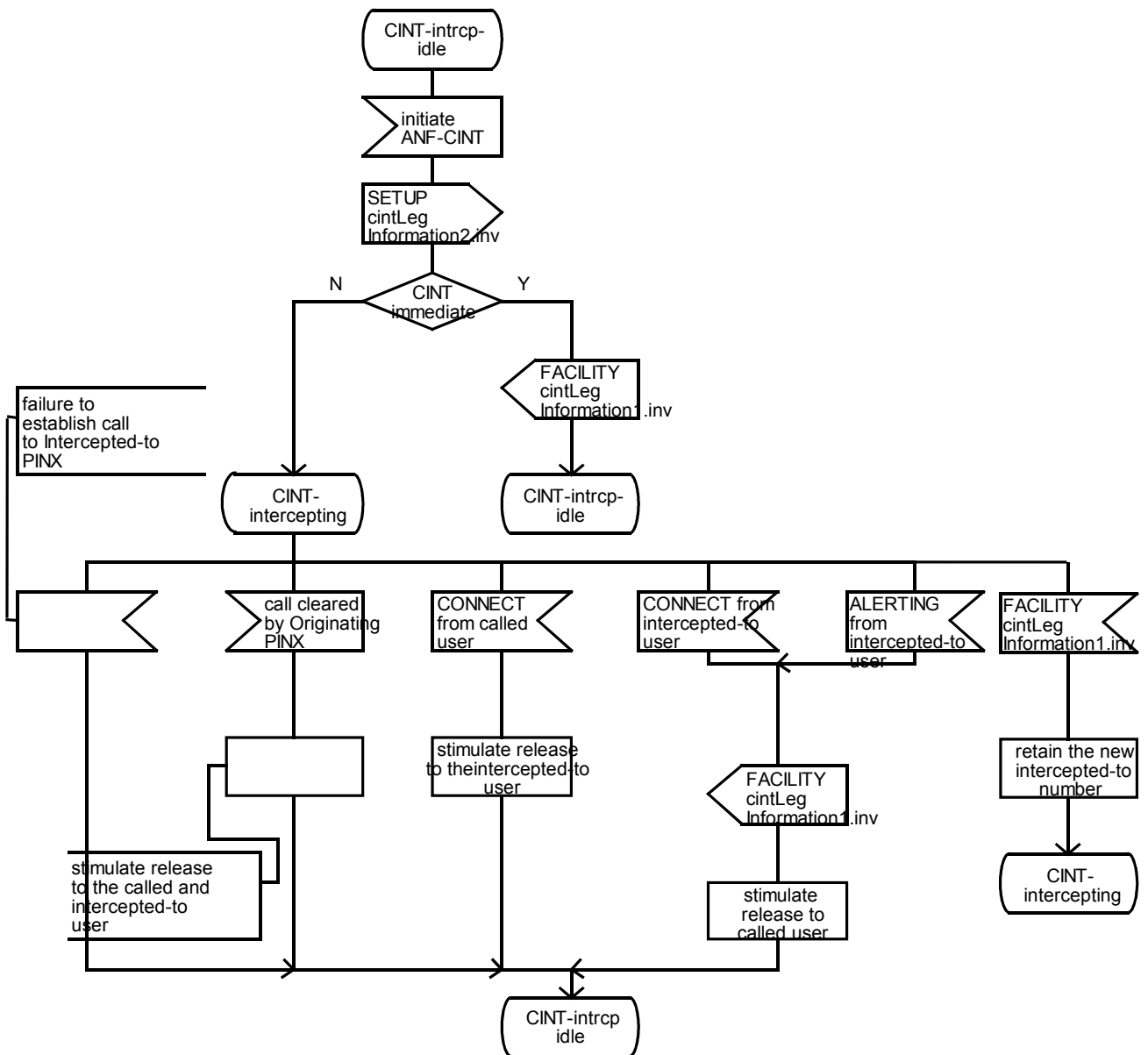
Figure C.2 - SDL Representation of ANF-CINT at the Intercepting PINX
