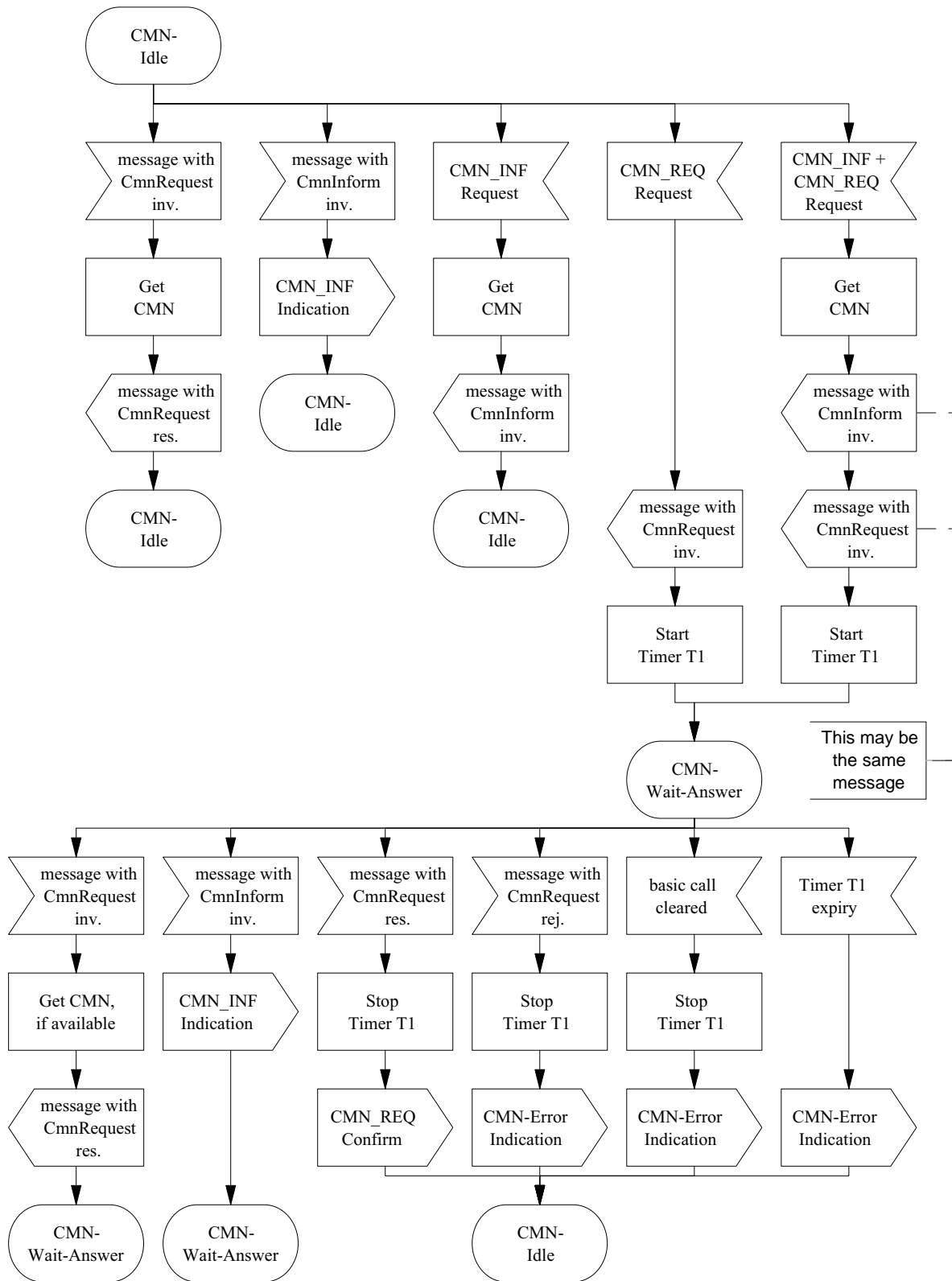
Figure C.2 - SDS Representation of ANF-CMN at the Terminating PINX
