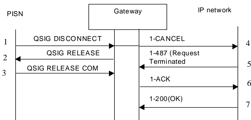
Figure 11 - Typical message sequence for call clearing from QSIG to SIP, during establishment of a call from QSIG to SIP (gateway has received a provisional response to the SIP INVITE request but not a final response)
