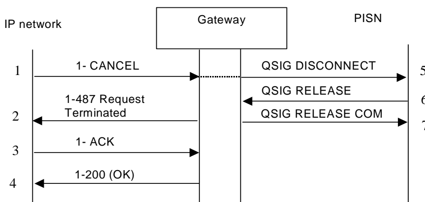
Figure 14 - Typical message sequence for call clearing from SIP to QSIG, during establishment of a call from SIP to QSIG (gateway has sent a provisional response to the SIP INVITE request but not a final response)
