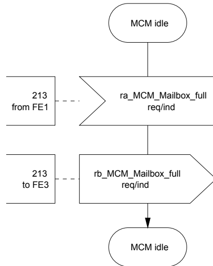
Figure 13g – SDL for MCM Mailbox-full Indication for FE2, Served User's control entity
