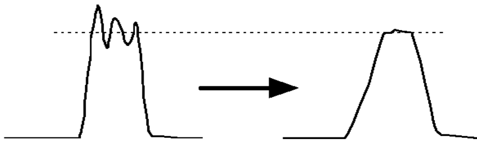
Figure U.3a - Elimination of ringing by LPF (~100 MHz)
