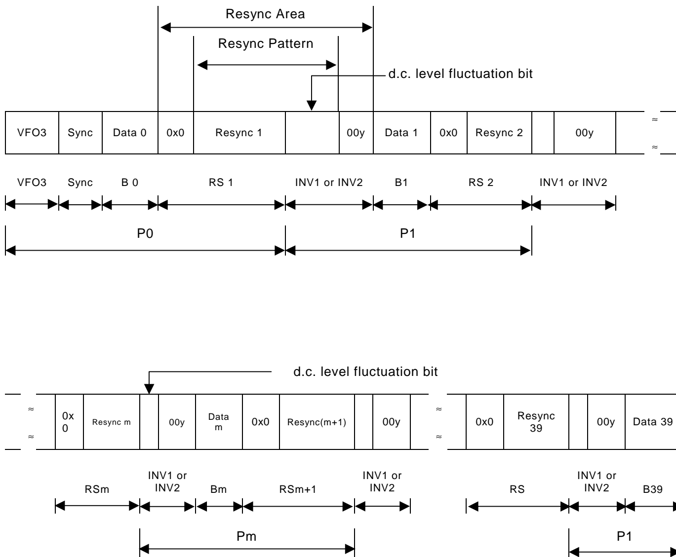
Figure F.1 - Example of Resync byte
