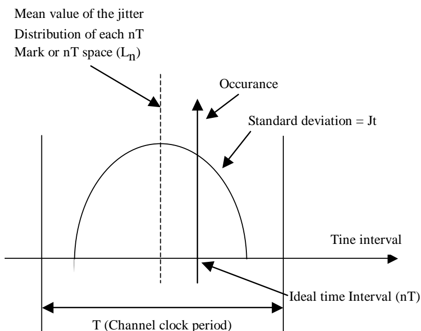
Figure H.3 - Measured distribution of timing jitter
