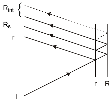
Figure D.1 — Reflectance calibration
