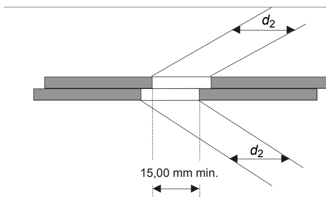
Figure 9 — Rim area
