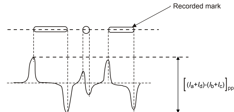
Figure 16 — Differential phase tracking error signal
