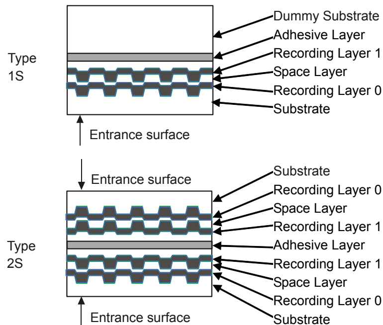
Figure 1 — Disk outline
