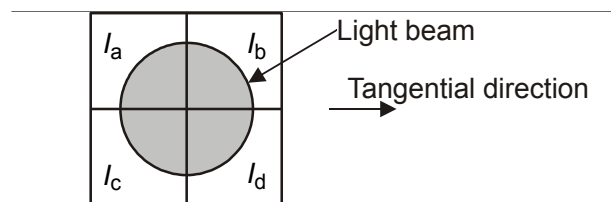
Figure 15 — Quadrant photo detector
