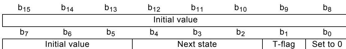
Figure 66 — DSV field
