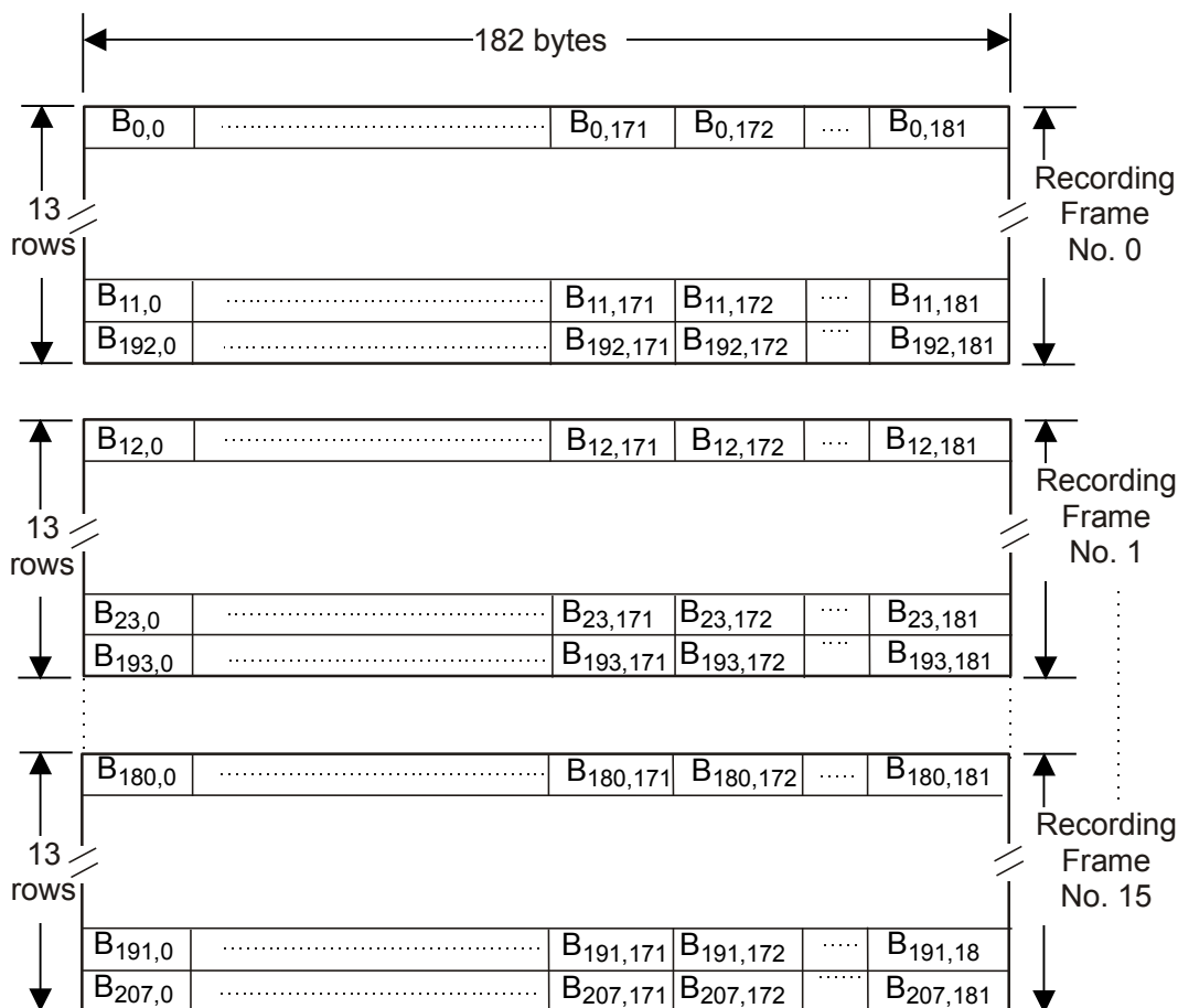
Figure 31 — Recording Frames obtained from an ECC Block
