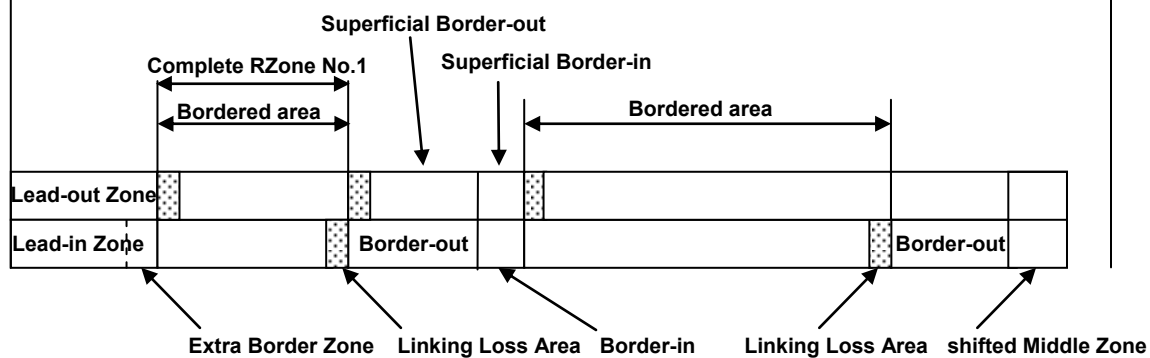
Figure L.2 — Examples of Border Recording in Information Zone
