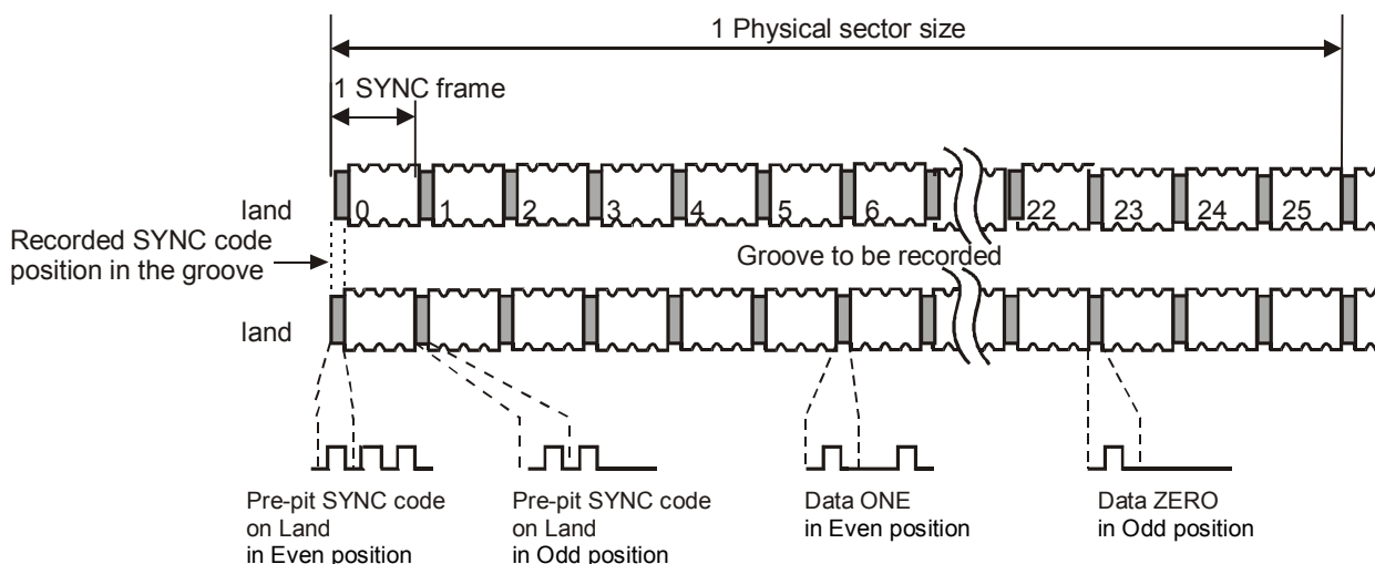
Figure 45 — Track formation
