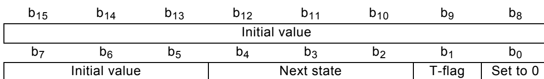
Figure 65 — DSV field
