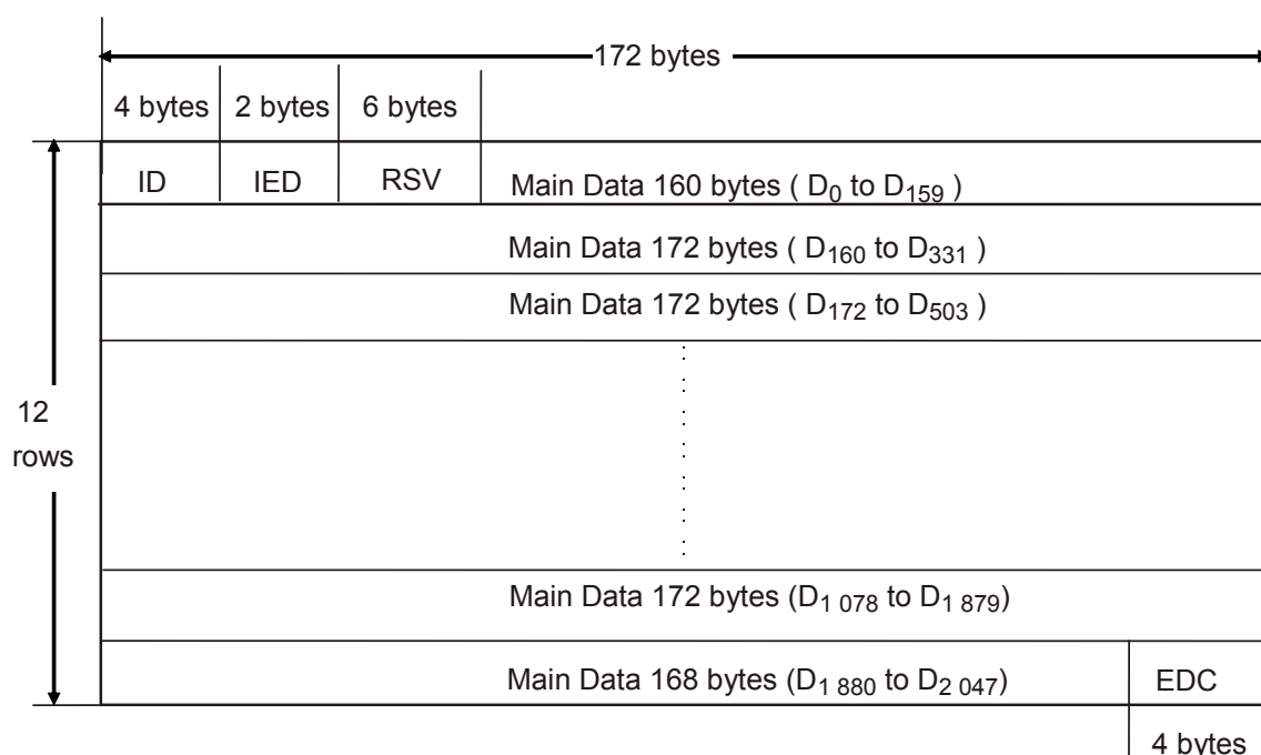
Figure 26 — Data Frame
