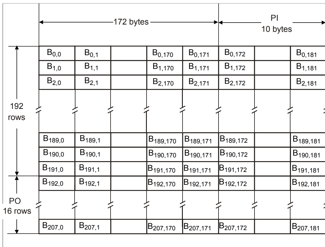
Figure 30 — ECC Block
