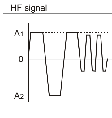
Figure H.1 — \beta < 0 (Low power)
