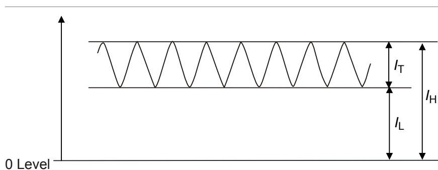
Figure 13 — Modulated amplitude
