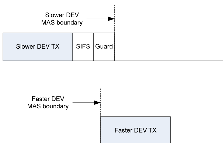
Figure 11 — Guard Time
