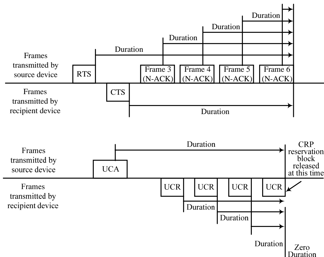
Figure 8 — Duration examples
