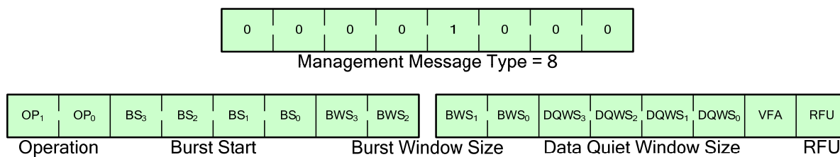
Figure 20 — BR-RSP message format
