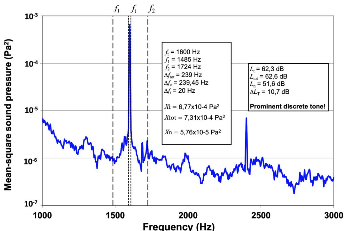
Figure A.1 — Tone-to-noise ratio method applied to a single tone in a critical band
