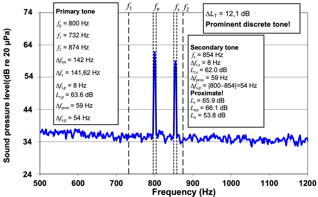
Figure 3 — Tone-to-noise ratio method applied to multiple tones in a critical band
