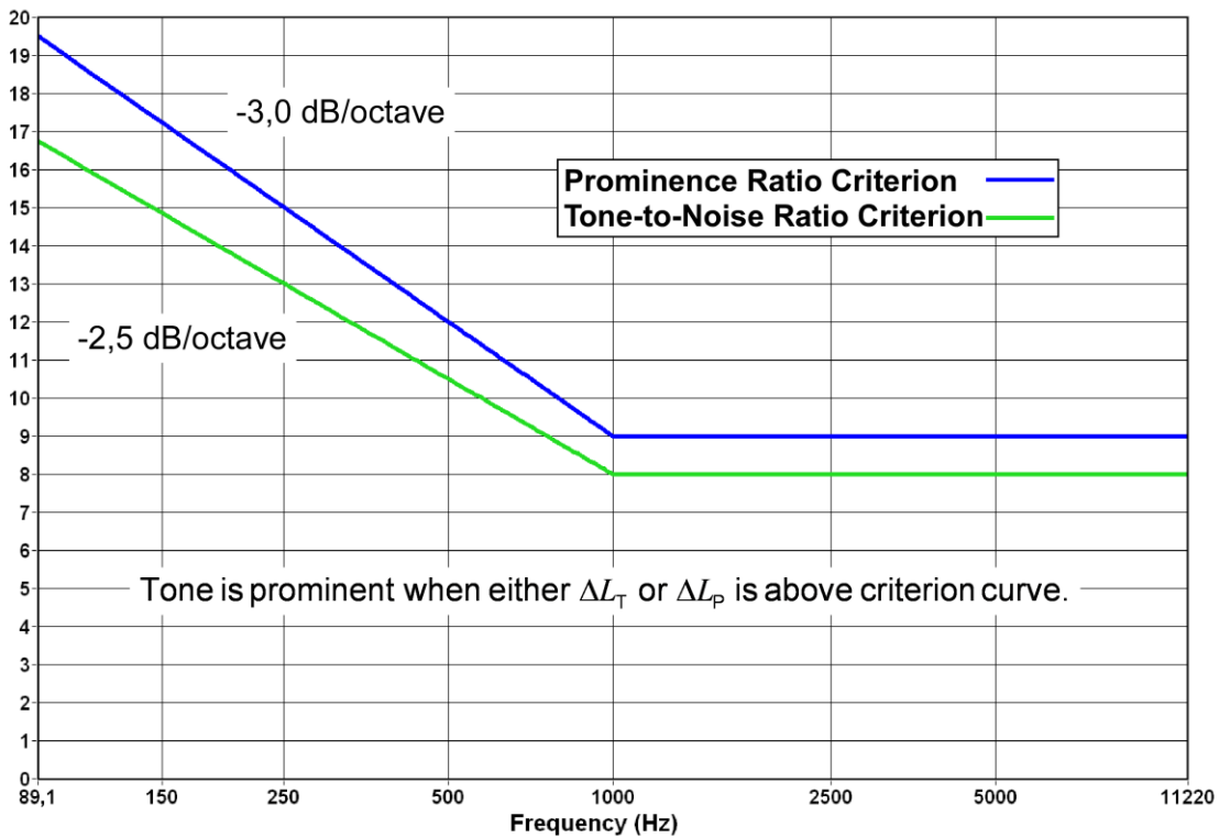
Figure 5 — Criteria for prominence for both tone-to-noise ratio (11.6) and prominence ratio (12.7) as a function of frequency
