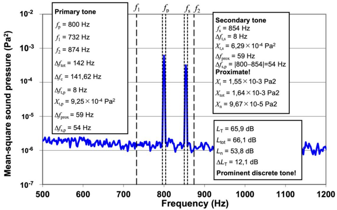
Figure A.2 — Tone-to-noise ratio method applied to multiple tones in a critical band
