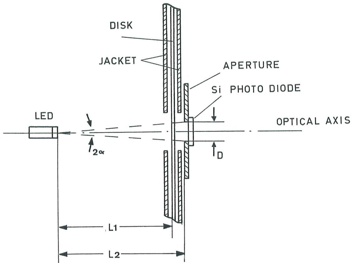
FIG. 1 MEASURING DEVICE
